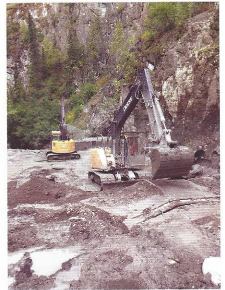
Tundra mats in use to allow machinery to operate on unstable sediments.
